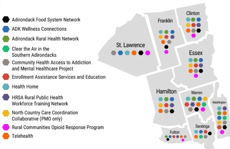
Figure 2: AHI Programs
